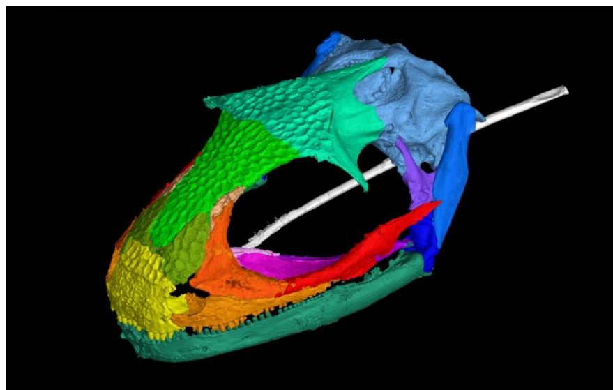
Most fossil albanerpetontids are crushed or in disarray. This CT image shows an exquisitely preserved adult albanerpetontid skull that is helping researchers re-envision these extinct amphibians. Credit: Edward Stanley/Florida Museum of Natural History/VGStudioMax3.4
