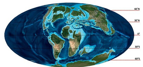
Paleogeography of the late Turonian (90 Ma)
